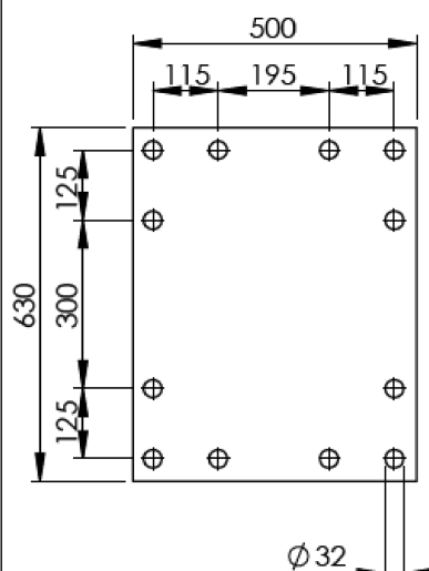
Gatenpatroon/hole pattern/ Bohrbild/motif de trous
